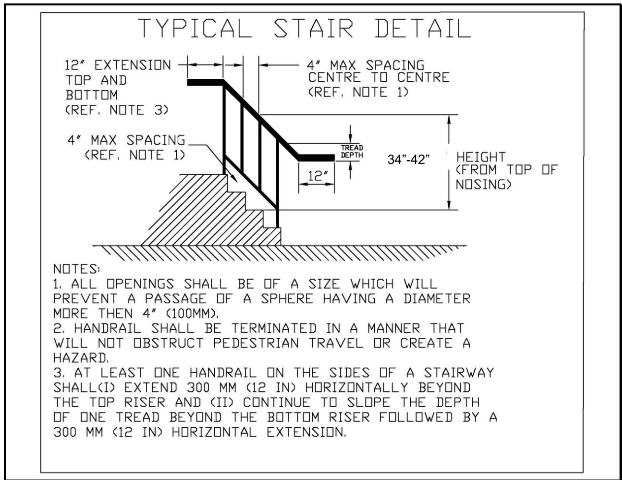
Figure 2: Typical Stair Detail (Side View) (Refer to Stair Design Criteria and Figure 3 for Additional Information)
